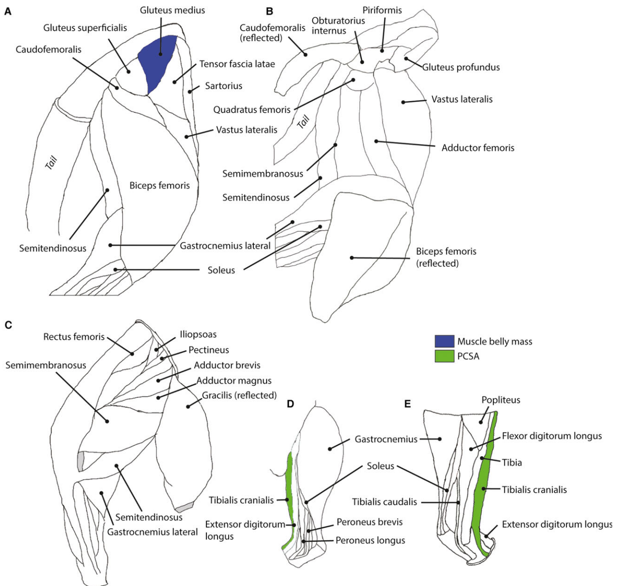
Fig. 2 Muscles displaying potential allometry (after phylogenetic analysis) in the studied felid species are shown in colour; others as white; for a representative right hindlimb. (A) Lateral superficial muscles of hip and knee. (B) Lateral, deeper muscles of the hindlimb. (C) Medial muscles of the thigh and shank. (D) Lateral muscles of the lower leg. (E) Medial muscles of the lower leg. Navy blue = muscle mass; green = PCSA. Stippling pattern is for negative allometry.
