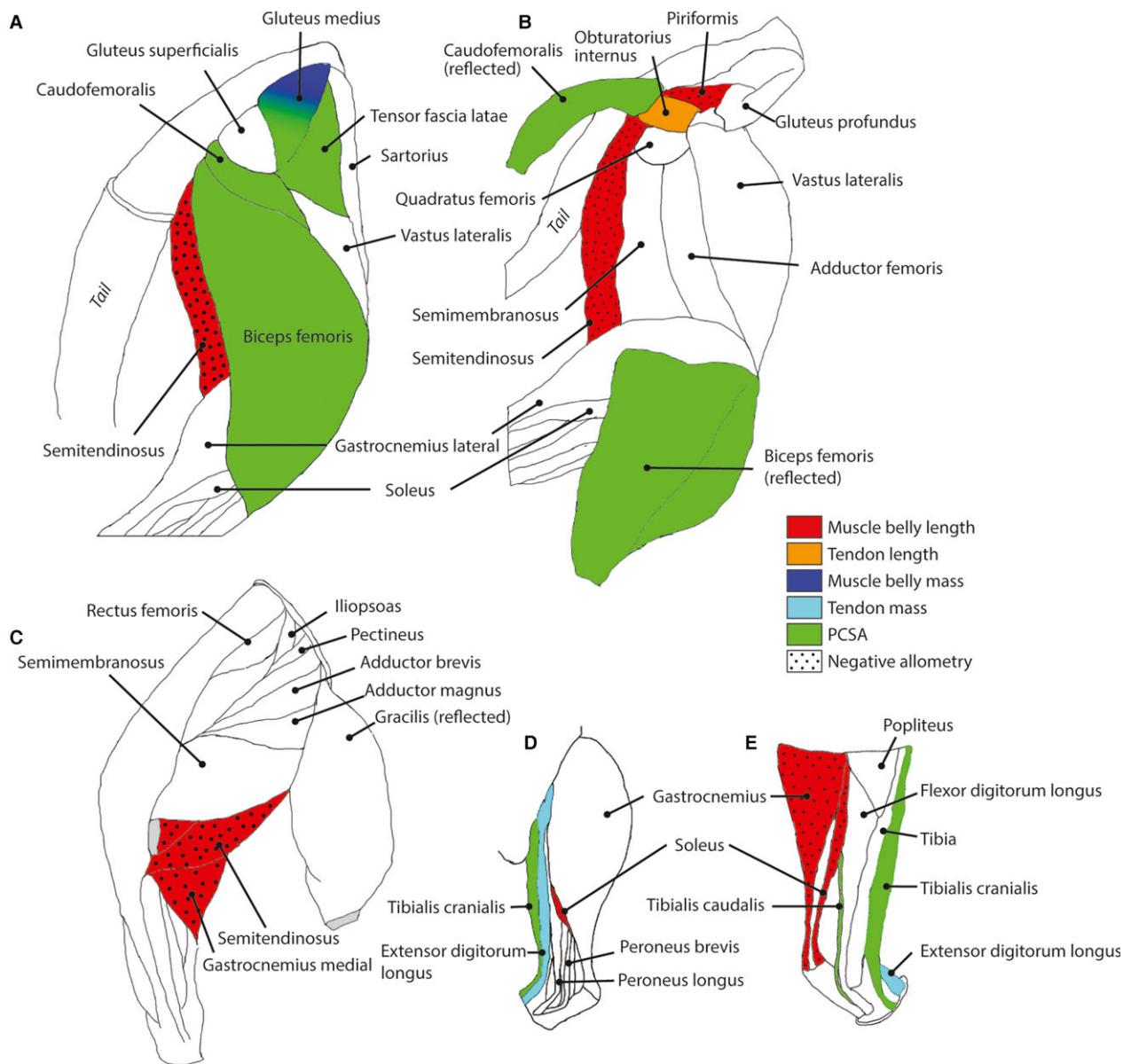
Fig. 1 Muscles displaying potential allometry (prior to phylogenetic analysis) in the studied felid species are shown in colour; others as white; for a representative right hindlimb. (A) Lateral superficial muscles of hip and knee. (B) Lateral, deeper muscles of the hindlimb. (C) Medial muscles of the thigh and shank. (D) Lateral muscles of the lower leg. (E) Medial muscles of the lower leg. Red = muscle belly length; orange = tendon length; navy blue = muscle mass; light blue = tendon mass; green = PCSA. Stippling pattern is for negative allometry. Muscles not shown: M. psoas majorum (Table 6); M. vastus intermedius (Tables 4 and 5); M. lateral digital extensor (Table 4); M. superficial digital flexor (Table 6); M. peroneus brevis (Table 2).
